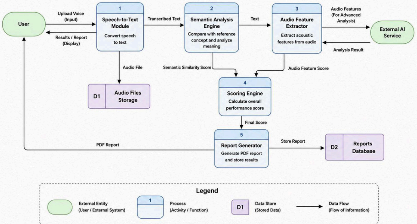
Figure 1: Data Flow Diagram
